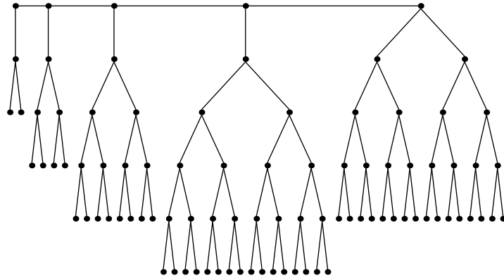
Festoon Tree for d = 2, n = 91
