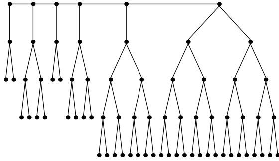
Festoon Tree for d = 2, n = 71
