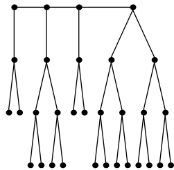
Festoon Tree for d = 2, n = 31
