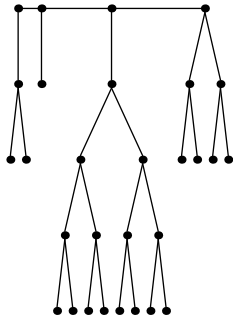
Festoon Tree for d = 2, n = 29
