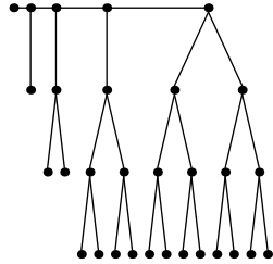
Festoon Tree for d = 2, n = 30
