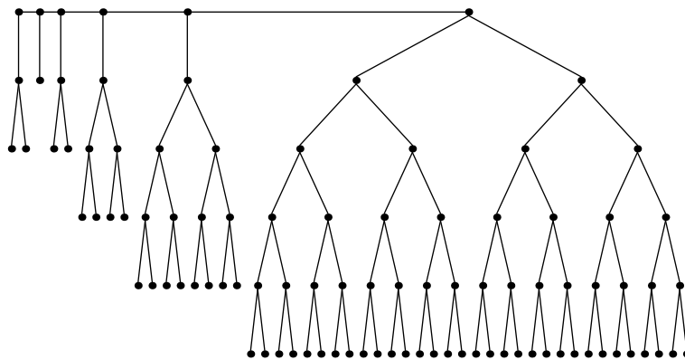
Festoon Tree for d = 2, n = 96
