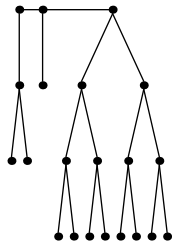
Festoon Tree for d = 2 , n = 21
