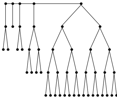
Festoon Tree for d = 2, n = 49
