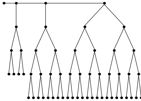
Festoon Tree for d = 2, n = 56
