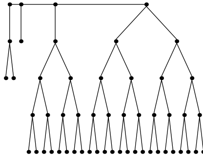
Festoon Tree for d = 2, n = 53
