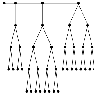
Festoon Tree for d = 2, n = 40
