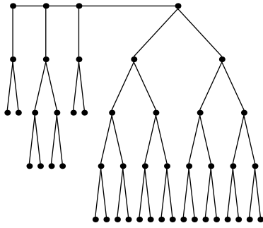
Festoon Tree for d = 2, n = 47
