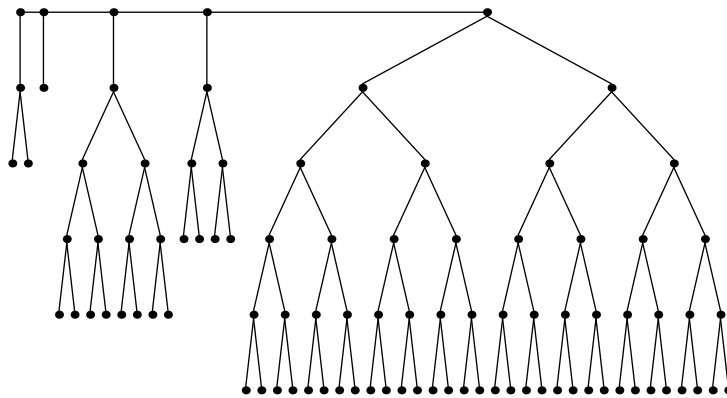
Festoon Tree for d = 2, n = 93
