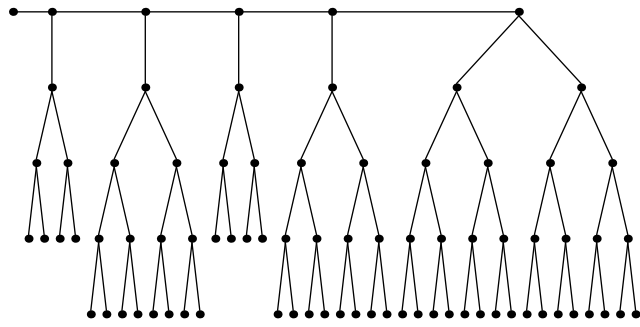
Festoon Tree for d = 2, n = 80
