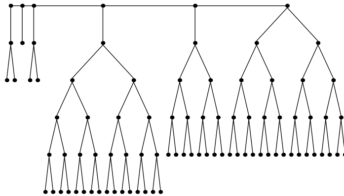
Festoon Tree for d = 2, n = 89
