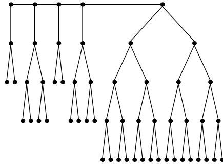
Festoon Tree for d = 2, n = 55
