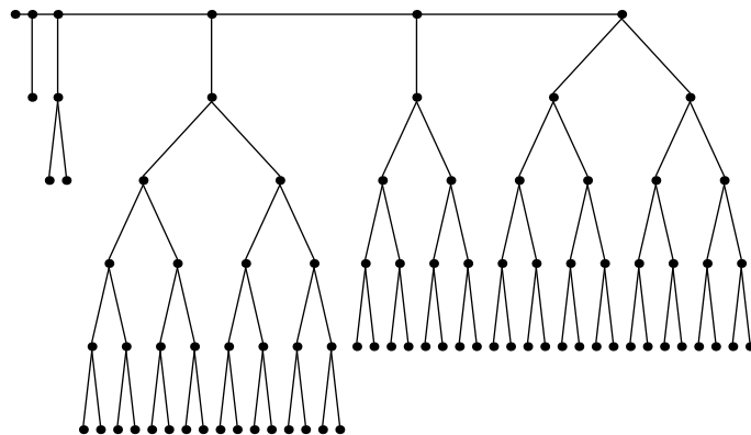
Festoon Tree for d = 2, n = 86
