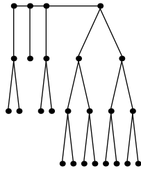
Festoon Tree for d = 2, n = 25
