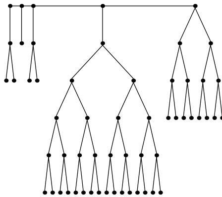
Festoon Tree for d = 2, n = 57
