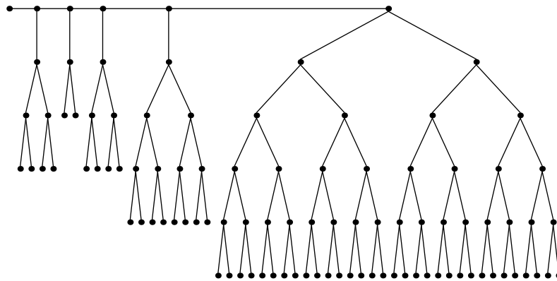
Festoon Tree for d = 2, n = 100
