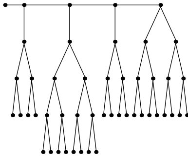
Festoon Tree for d = 2, n = 48
