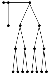
Festoon Tree for d = 2 , n = 18
