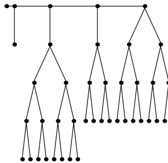
Festoon Tree for d = 2, n = 42
