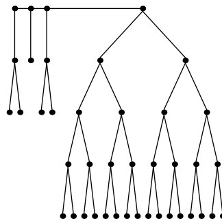
Festoon Tree for d = 2, n = 41
