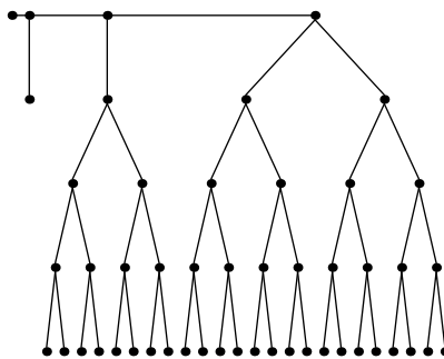
Festoon Tree for d = 2, n = 50
