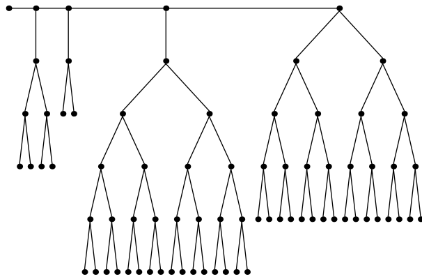
Festoon Tree for d = 2, n = 76
