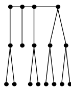
Festoon Tree for d = 2, n = 17
