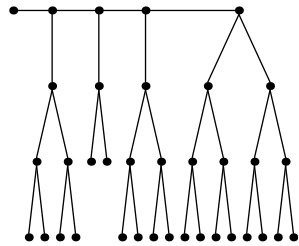
Festoon Tree for d = 2, n = 36
