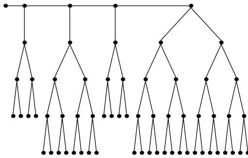
Festoon Tree for d = 2, n = 64
