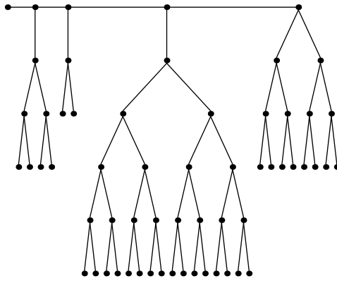
Festoon Tree for d = 2, n = 60
