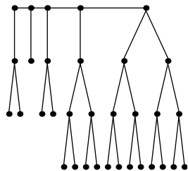
Festoon Tree for d = 2, n = 33
