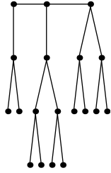
Festoon Tree for d = 2 , n = 19
