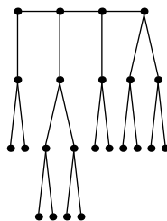
Festoon Tree for d = 2 , n = 22
