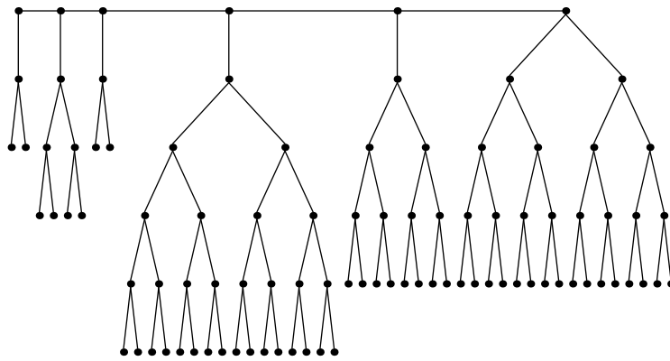
Festoon Tree for d = 2, n = 95
