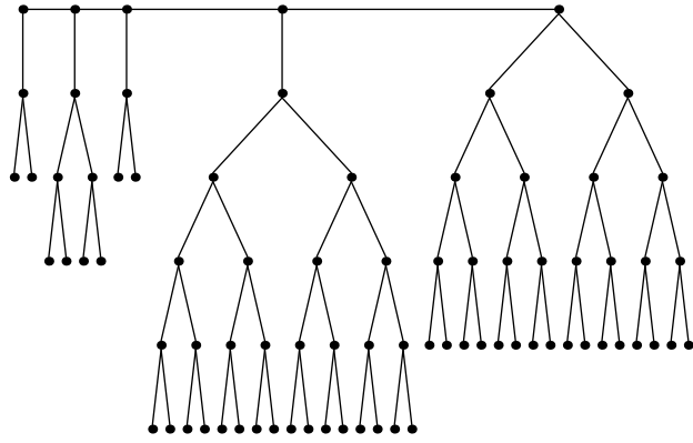
Festoon Tree for d = 2, n = 79
