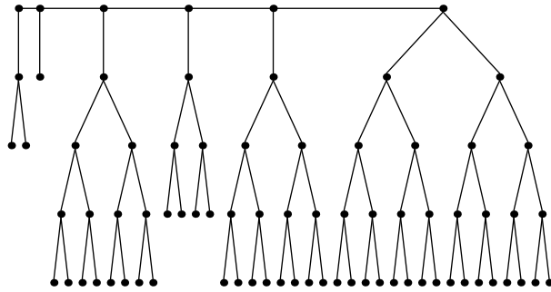
Festoon Tree for d = 2, n = 77
