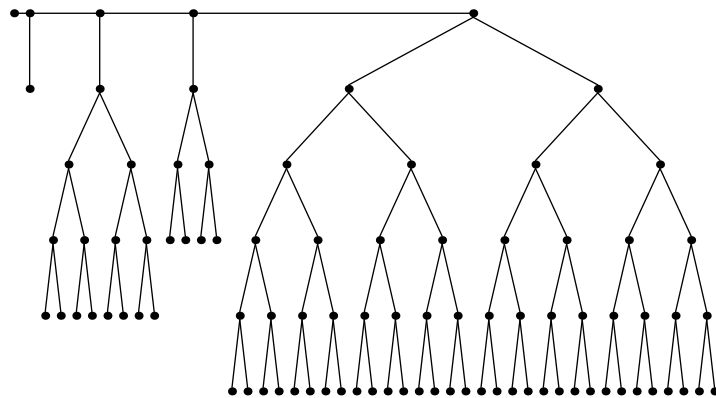
Festoon Tree for d = 2, n = 89
