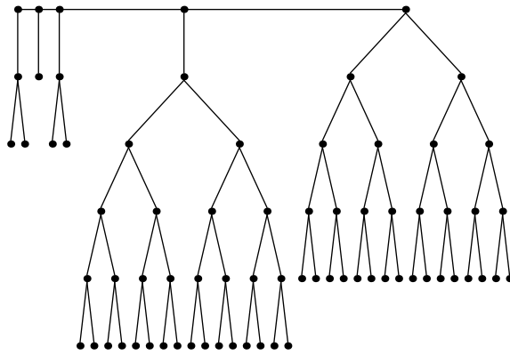
Festoon Tree for d = 2, n = 73
