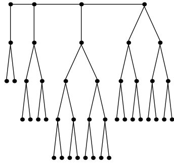
Festoon Tree for d = 2, n = 43
