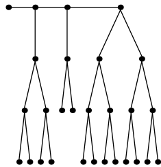
Festoon Tree for d = 2, n = 28
