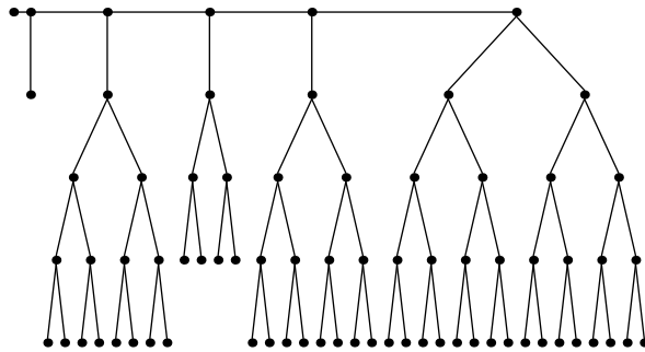
Festoon Tree for d = 2, n = 74
