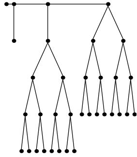
Festoon Tree for d = 2, n = 34
