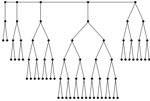
Festoon Tree for d = 2, n = 75
