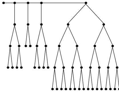
Festoon Tree for d = 2, n = 52
