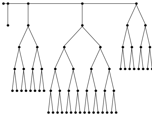
Festoon Tree for d = 2, n = 66
