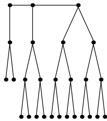
Festoon Tree for d = 2, n = 27
