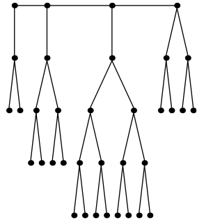
Festoon Tree for d = 2, n = 35
