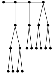
Festoon Tree for d = 2 , n = 20
