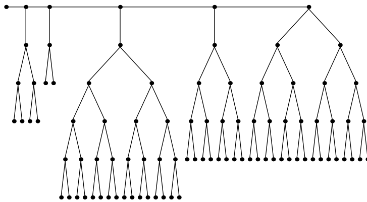
Festoon Tree for d = 2, n = 92
