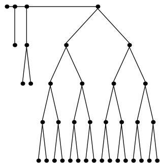
Festoon Tree for d = 2, n = 37
