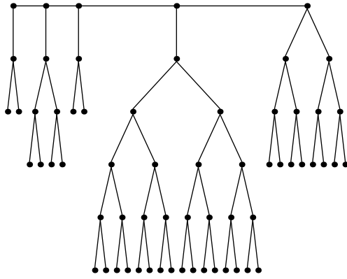
Festoon Tree for d = 2, n = 63
