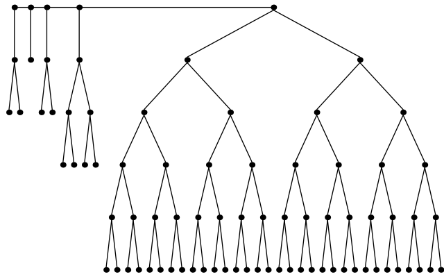
Festoon Tree for d = 2, n = 81
