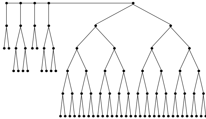
Festoon Tree for d = 2, n = 87
