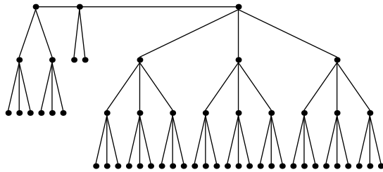
Festoon Tree for d = 3, n = 52
