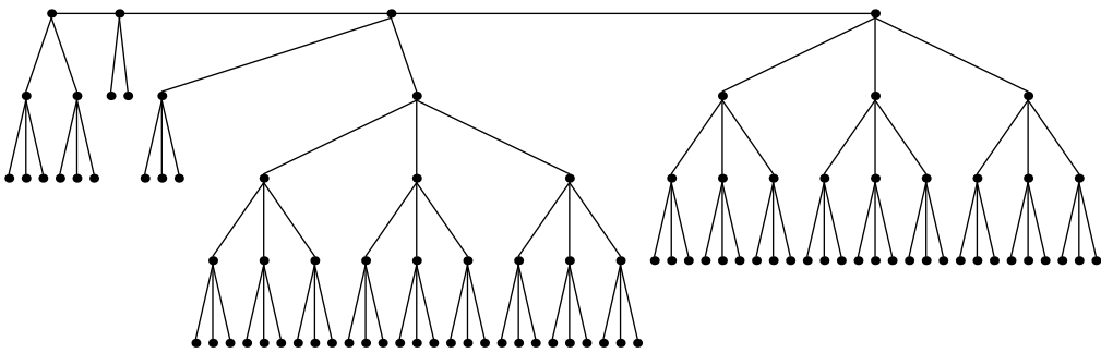
Festoon Tree for d = 3, n = 97
