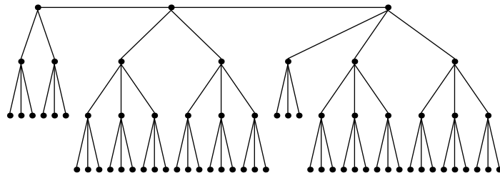
Festoon Tree for d = 3, n = 67
