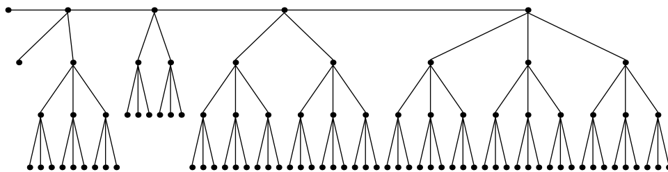
Festoon Tree for d = 3, n = 92
