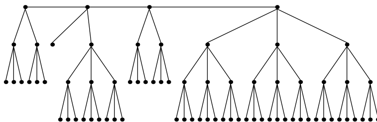
Festoon Tree for d = 3, n = 73
