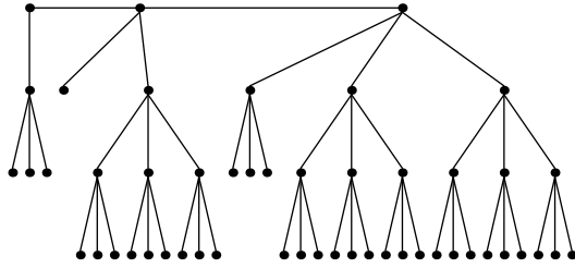
Festoon Tree for d = 3, n = 51
