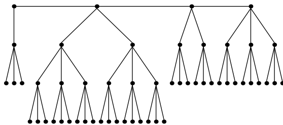
Festoon Tree for d = 3, n = 53
