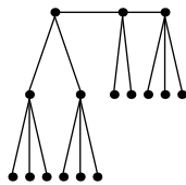
Festoon Tree for d = 3, n = 16
