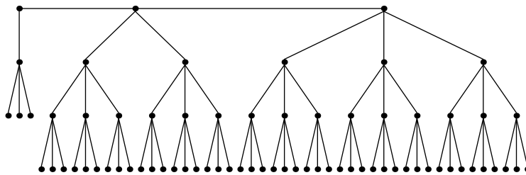
Festoon Tree for d = 3, n = 72
