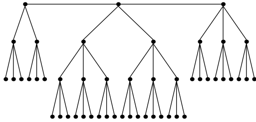
Festoon Tree for d = 3, n = 49
