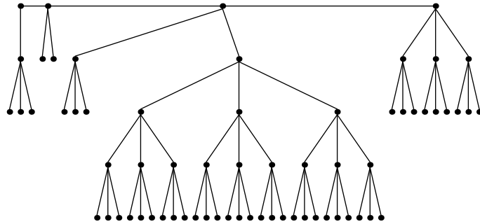
Festoon Tree for d = 3, n = 66
