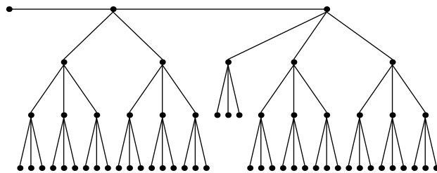
Festoon Tree for d = 3, n = 59
