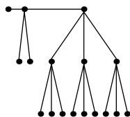
Festoon Tree for d = 3, n = 17
