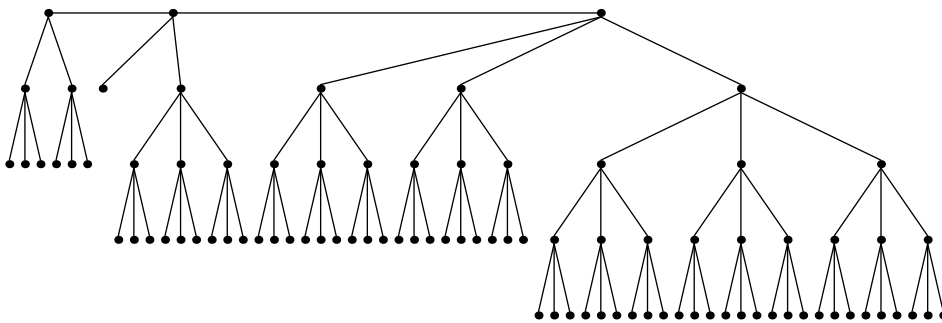
Festoon Tree for d = 3, n = 91
