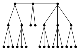
Festoon Tree for d = 3, n = 25
