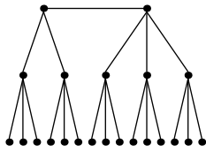
Festoon Tree for d = 3, n = 22
