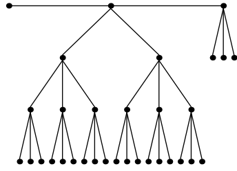
Festoon Tree for d = 3, n = 32
