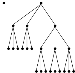
Festoon Tree for d = 3, n = 23
