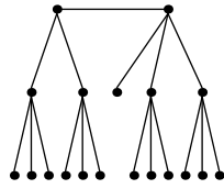
Festoon Tree for d = 3, n = 19
