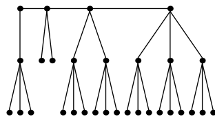
Festoon Tree for d = 3, n = 30
