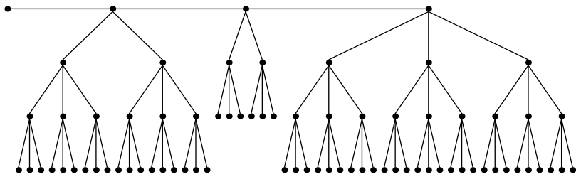
Festoon Tree for d = 3, n = 77
