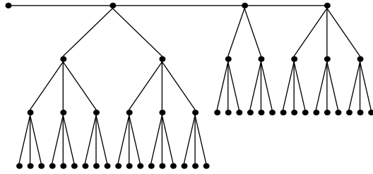
Festoon Tree for d = 3, n = 50
