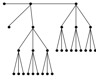
Festoon Tree for d = 3, n = 29
