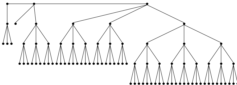
Festoon Tree for d = 3, n = 87
