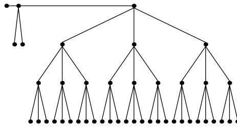
Festoon Tree for d = 3, n = 44
