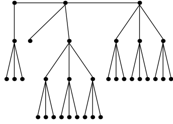
Festoon Tree for d = 3, n = 33
