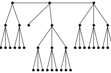
Festoon Tree for d = 3, n = 37
