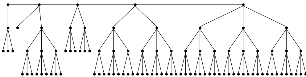
Festoon Tree for d = 3, n = 96
