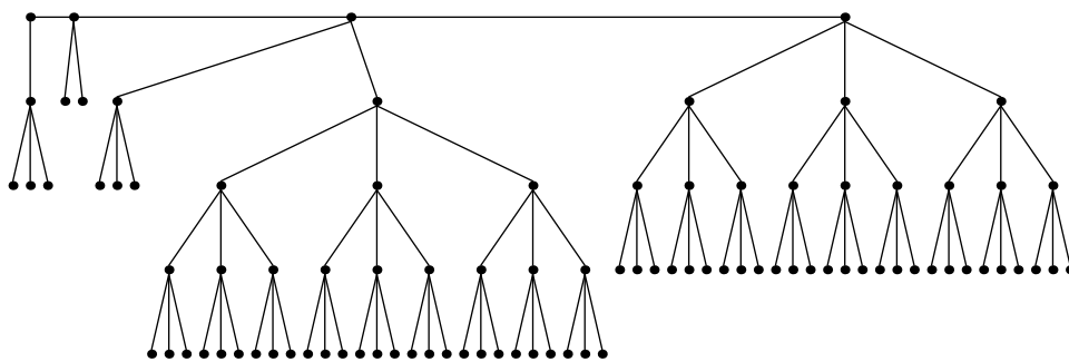
Festoon Tree for d = 3, n = 93
