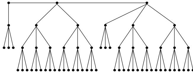
Festoon Tree for d = 3, n = 63
