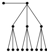
Festoon Tree for d = 3, n = 14
