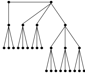
Festoon Tree for d = 3, n = 27
