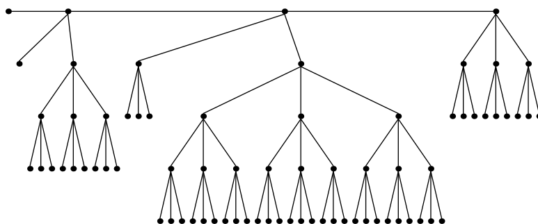
Festoon Tree for d = 3, n = 74
