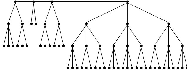
Festoon Tree for d = 3, n = 61
