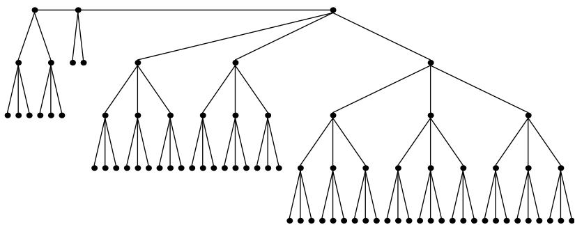
Festoon Tree for d = 3, n = 79
