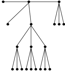
Festoon Tree for d = 3, n = 20
