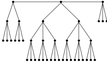
Festoon Tree for d = 3, n = 40
