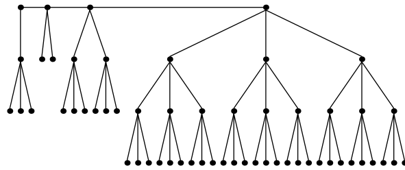
Festoon Tree for d = 3, n = 57
