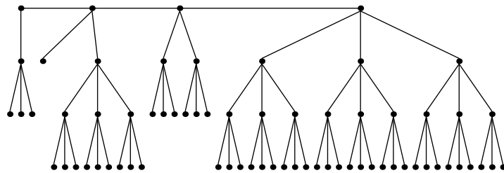
Festoon Tree for d = 3, n = 69
