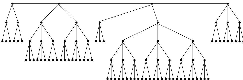
Festoon Tree for d = 3, n = 93
