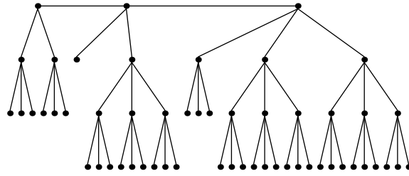
Festoon Tree for d = 3, n = 55
