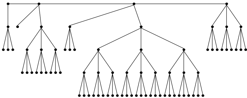
Festoon Tree for d = 3, n = 78
