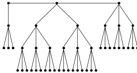
Festoon Tree for d = 3, n = 45
