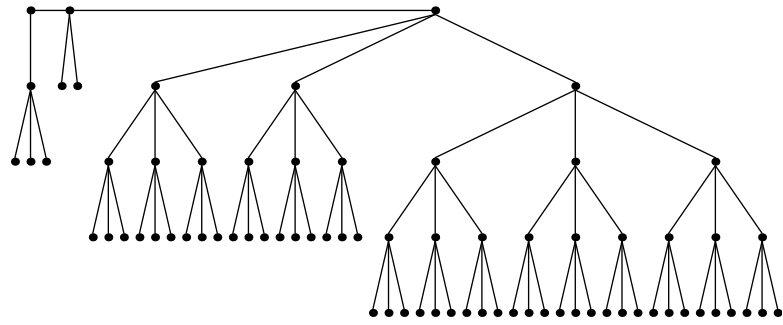
Festoon Tree for d = 3, n = 75
