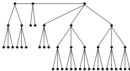
Festoon Tree for d = 3, n = 42
