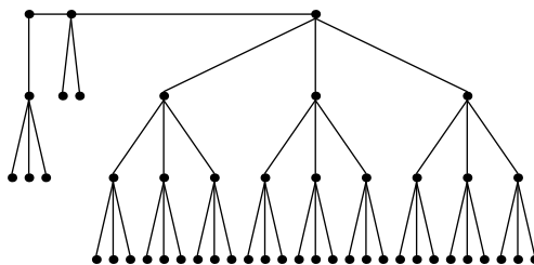
Festoon Tree for d = 3, n = 48
