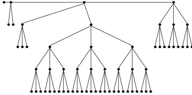
Festoon Tree for d = 3, n = 62
