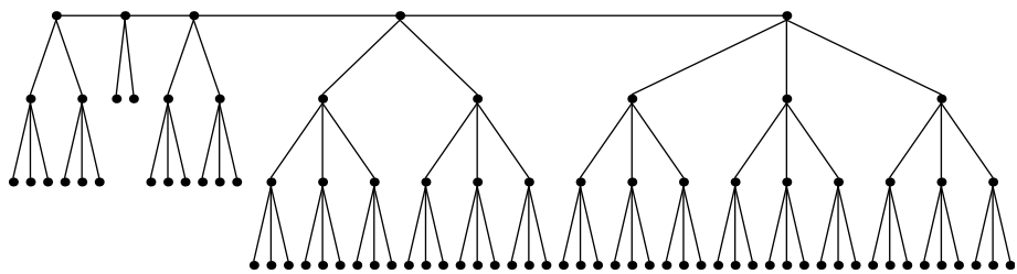
Festoon Tree for d = 3, n = 88
