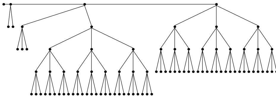
Festoon Tree for d = 3, n = 89
