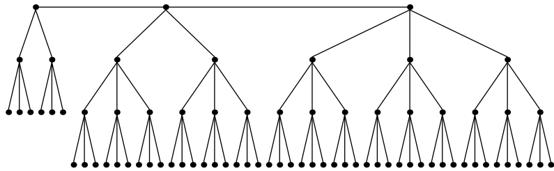
Festoon Tree for d = 3, n = 76
