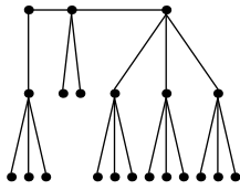
Festoon Tree for d = 3, n = 21
