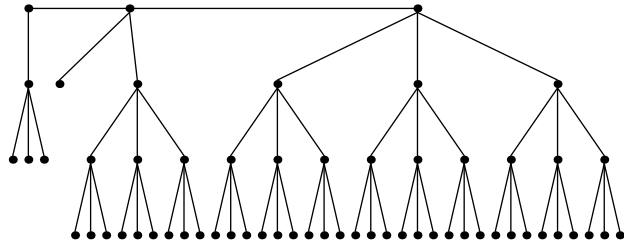
Festoon Tree for d = 3, n = 60
