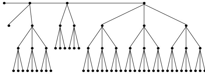
Festoon Tree for d = 3, n = 65
