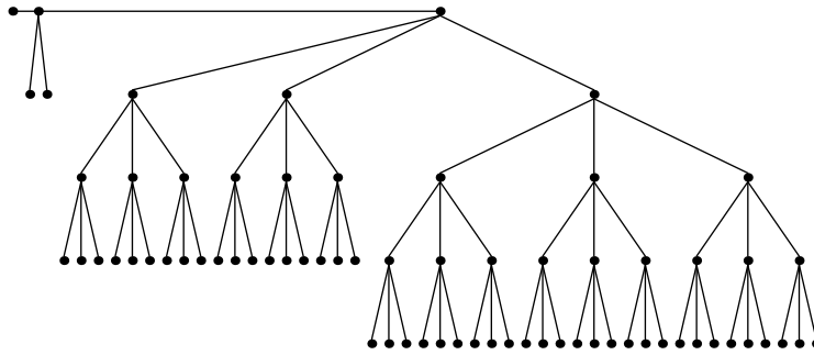
Festoon Tree for d = 3, n = 71
