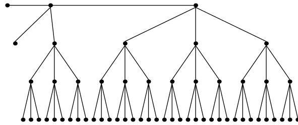
Festoon Tree for d = 3, n = 56
