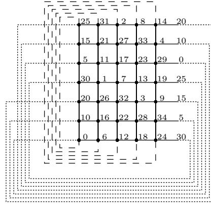
(a) C_{35}(6, 10)
